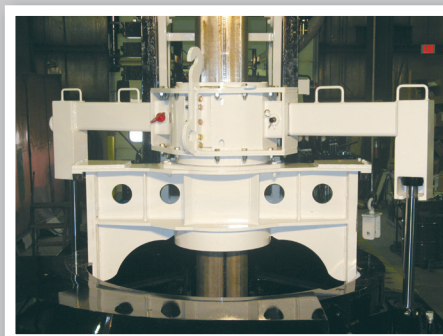
Pull down assembly
